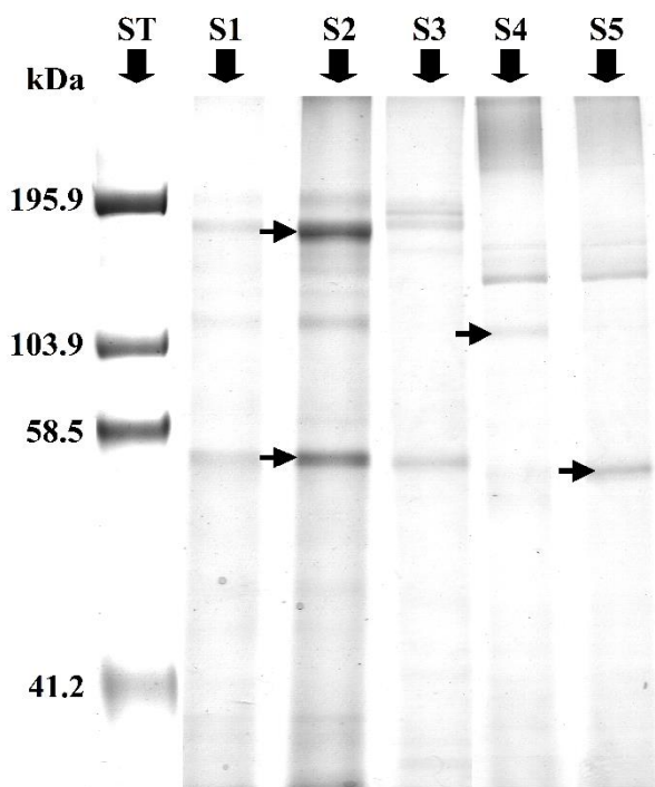
Figure 2. SDS-poly acrylamide gel electrophoresis profiles of copepod samples containing between 79 and up to 290 \mu\text{g mL}^{-1} of the total soluble proteins. Lanes: ST (protein standards with molecular sizes shown in kDa), S1 (females fed P. minimum ), S2 (females fed T. rotula ), S3 (males after-samplings preserved), S4 (eggs produced on P. minimum ) and S5 (eggs produced on T. rotula ). Black arrows highlight some specific electrophoretic bands: 167 and 56-kDa in S2, 113-kDa in S4, and 56-kDa in S5.
