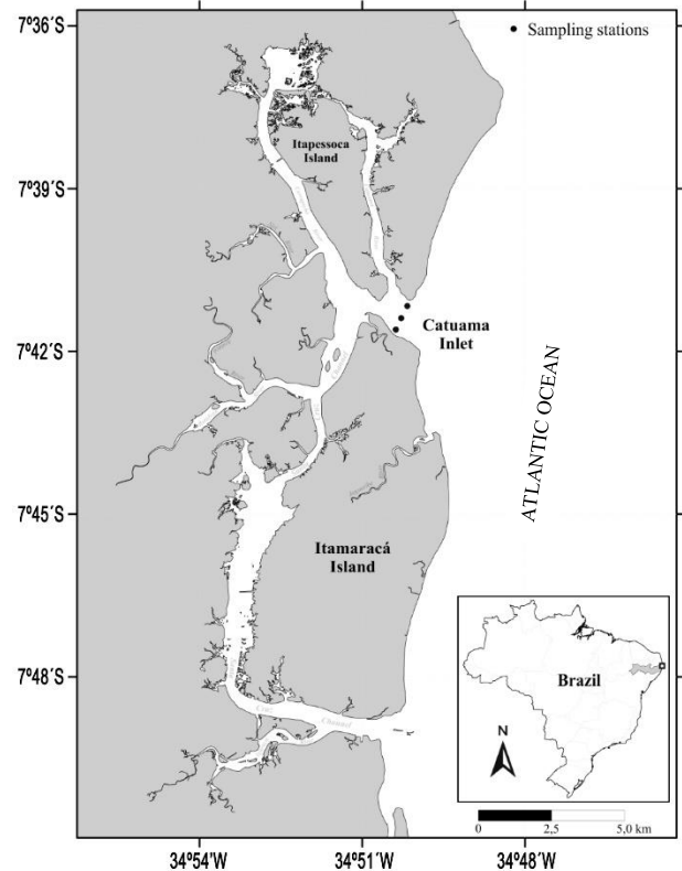
Figure 1. Itamaracá estuarine system (Pernambuco, Brazil) showing the Catuama Inlet and the sampling stations.
