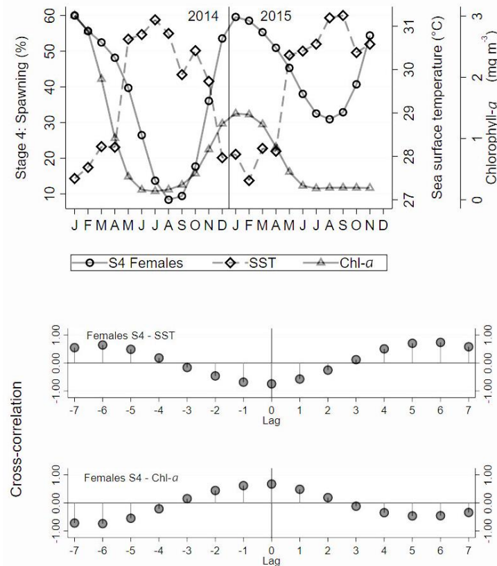
Figure 8. Smoothed frequency of spawning (S4) females, sea surface temperature (SST), and chlorophyll- a concentration (Chl- a ) along the study period and cross-correlation correlograms for S4-SST and S4-Chl- a .
