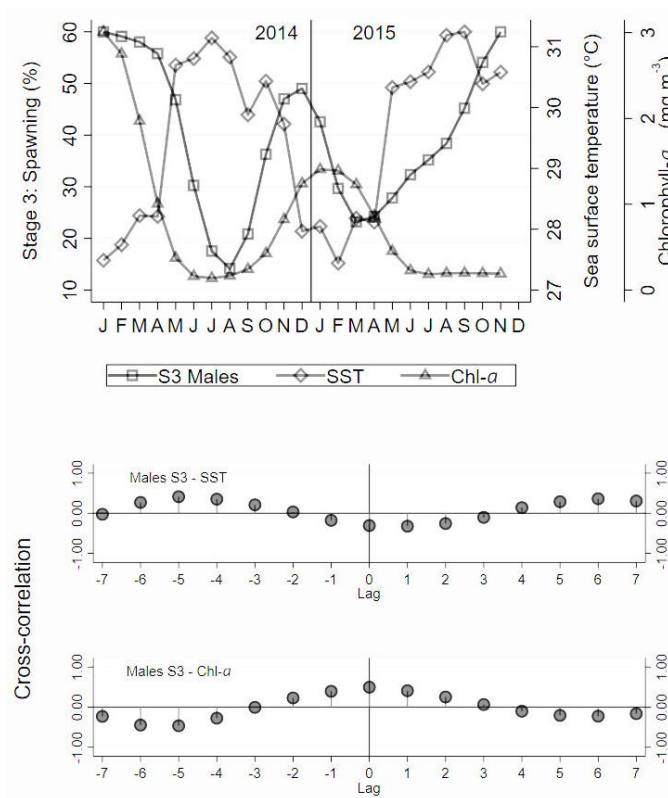
Figure 10. Smoothed frequency of spawning (S3) males, sea surface temperature (SST), and chlorophyll- a concentration (Chl- a ) along the study period and cross-correlation correlograms for S3-SST and S3-Chl- a .
