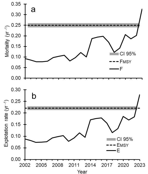
Figure 6. a) Fishing mortality (F) and mortality from maximum sustainable yield ( F_{MSY} ) and b) exploitation rate and exploitation rate from maximum sustainable yield ( E_{MSY} ), confidence intervals CI ( \alpha = 0.05 ), of Gulf corvina ( Cynoscion othonopterus ) in the Upper Gulf of California, during the period from 2002 to 2023.
