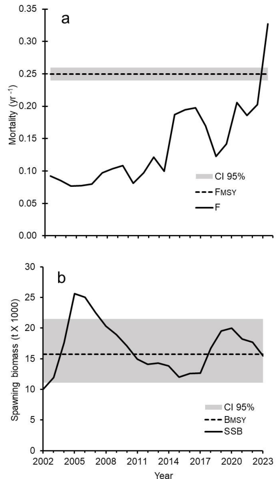
Figure 9. a) Interannual variation in fishing mortality (F) and b) spawning stock biomass (SSB), with reference points ( F_{MSY} and B_{MSY} ) and confidence intervals ( \alpha = 0.05 ) of Gulf corvina ( Cynoscion othonopterus ) in the Upper Gulf of California, during the period from 2002 to 2023.
