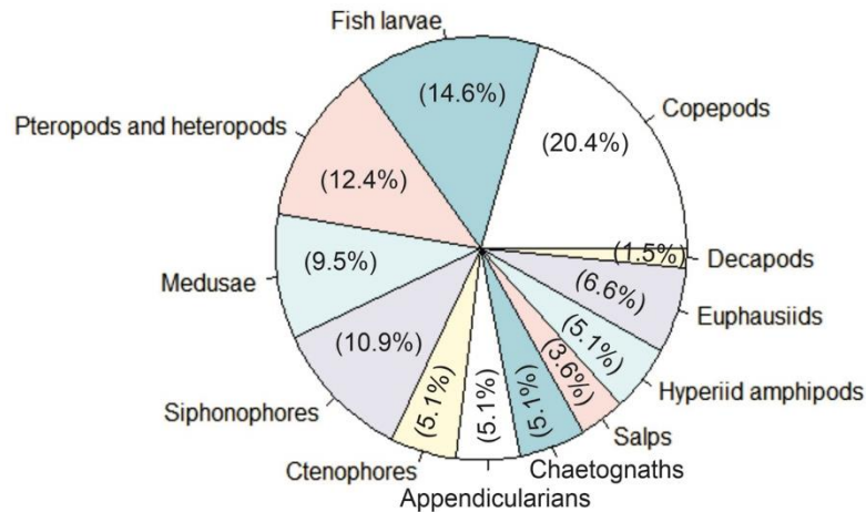
Figure 2. Research trends on marine zooplankton in the southern Gulf of Mexico (until August 2024). The figure highlights the need to focus research efforts on some zooplankton groups. The contribution of the studies for each group is indicated in percentage.
