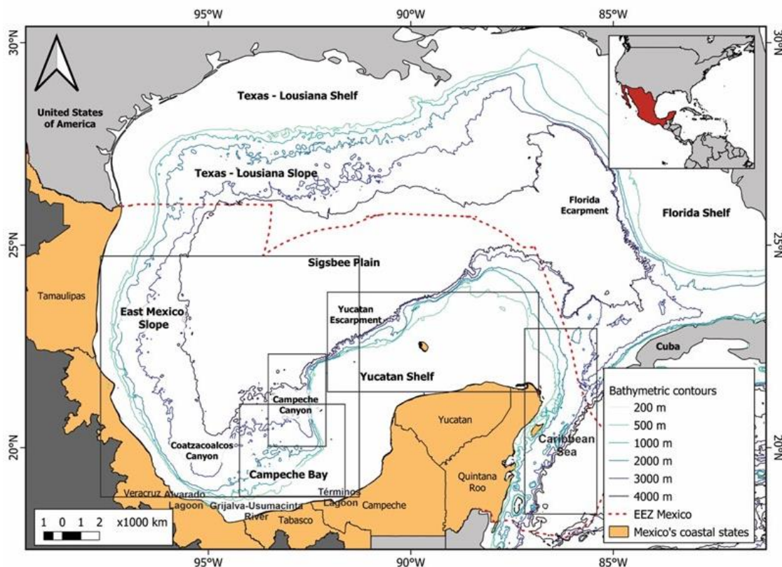
Figure 1. The Gulf of Mexico is a large marine ecosystem on the North American continent. The bathymetric contours are displayed in meters. The black boxes indicate areas with historical sampling coverage, including the Yucatan Shelf, the Campeche Canyon, the Campeche Bay, and, most recently, the deepwater regions of the gulf. Refer to the main text and Table 1 for a comprehensive overview of these sampling locations.
