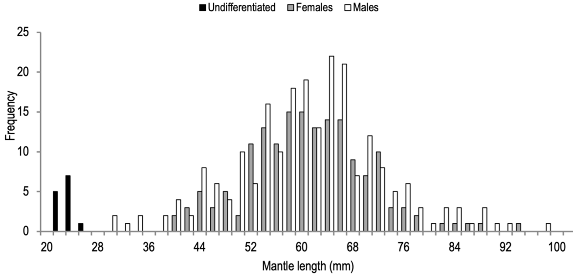
Figure 2. Size structure of Dosidicus gigas juveniles from the Gulf of Tehuantepec, April 2022. The arrows indicate the modes of the size classes: class I (11.0-29.9 mm mantle length, ML), class II (30.0-59.9 mm ML), and class III (60.0-99.9 mm ML).
