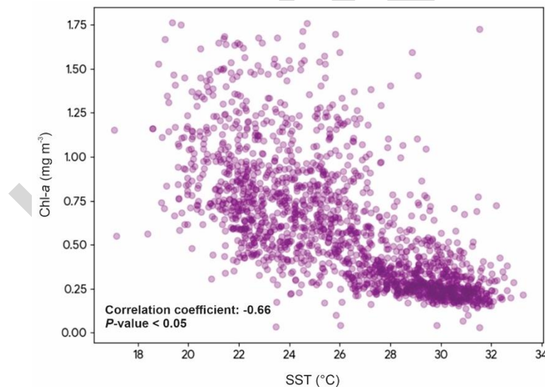
Figure 4. Pearson correlation analysis between sea surface temperature (SST, °C) and chlorophyll- a (Chl- a , mg m -3 ) concentration ( r = -0.66 , P\text{-value} < 0.05 ).
