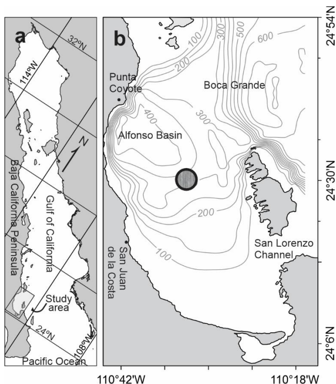
Figure 1. Location of a) the Gulf of California, Mexico; the rectangle represents the location of the Bay of La Paz; and b) the Bay of La Paz. The gray circle is ~4.4 km in diameter and centered at 24°30'N and 110°33'W; bathymetry is shown in meters.
