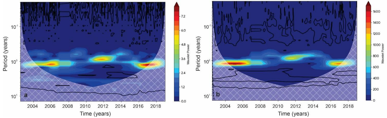
Figure 5. Continuous Wavelet Transform (Morlet) Power Spectrum of a) chlorophyll- a and b) sea surface temperature. The color bar represents wavelet power, with warmer colors indicating higher spectral power. The hatched, lighter region at the bottom represents the cone of influence, where edge effects may distort the spectrum. The black contour lines represent the 95% confidence level.
