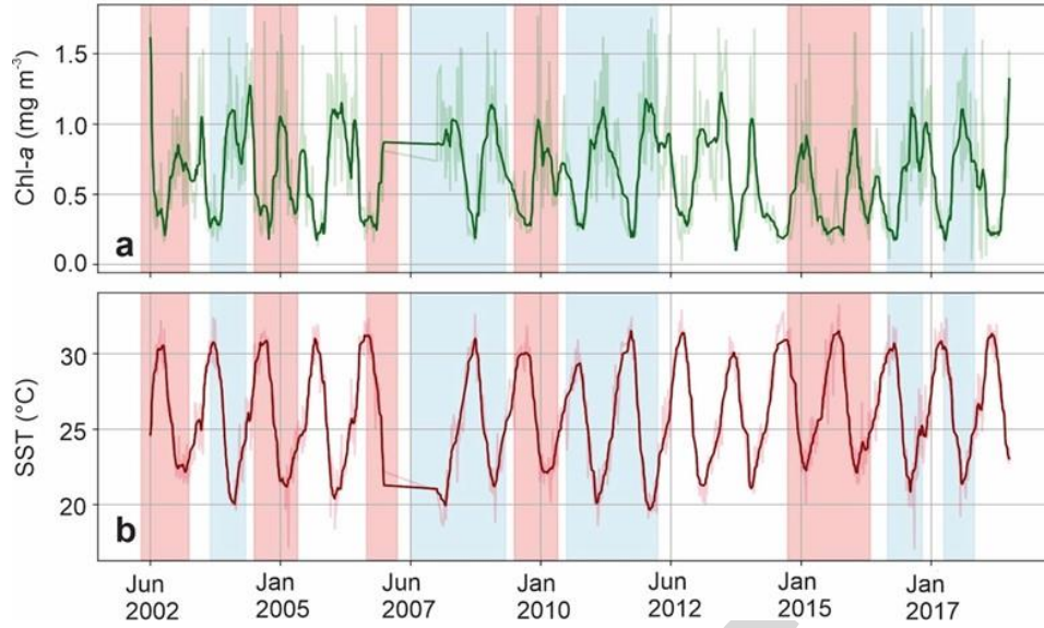
Figure 2. Time series from June 2002 to December 2018 of a) chlorophyll- a (Chl- a , \text{mg m}^{-3} ), the smoothed green line represents the outlier-removed time series, whereas the solid green line depicts the filtered data, and b) sea surface temperature (SST, ^{\circ}\text{C} ), the smoothed red line represents the outlier-removed time series, whereas the solid red line depicts the filtered data. See the Materials and Methods section for details. Shaded areas represent ENSO phases registered during the study period; red regions correspond to El Niño events and blue regions correspond to La Niña events.
