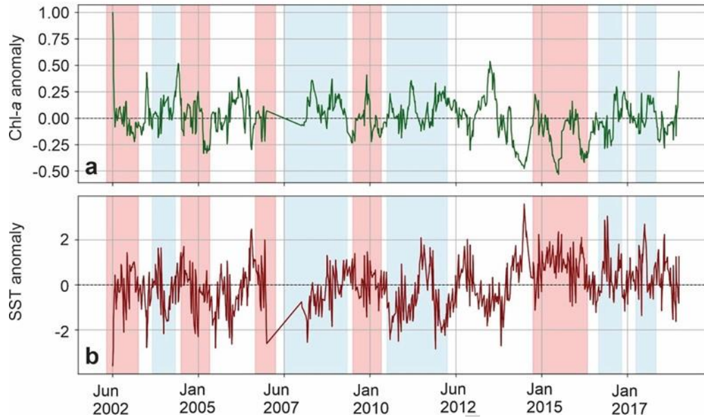
Figure 3. Anomalies calculated for a) chlorophyll- a (Chl- a ) concentration and b) sea surface temperature (SST) from June 2002 to December 2018. Shaded areas represent ENSO phases registered during the study period; red regions correspond to El Niño events and blue regions correspond to La Niña events.
